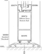
E Typical Threshold Detail
