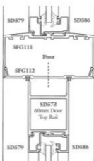
E Typical Threshold Detail
